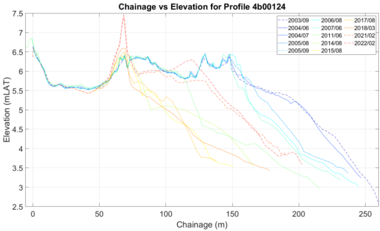
Plate 1.25 Profile 4b000124 elevation change (ABPmer, 2024b)
