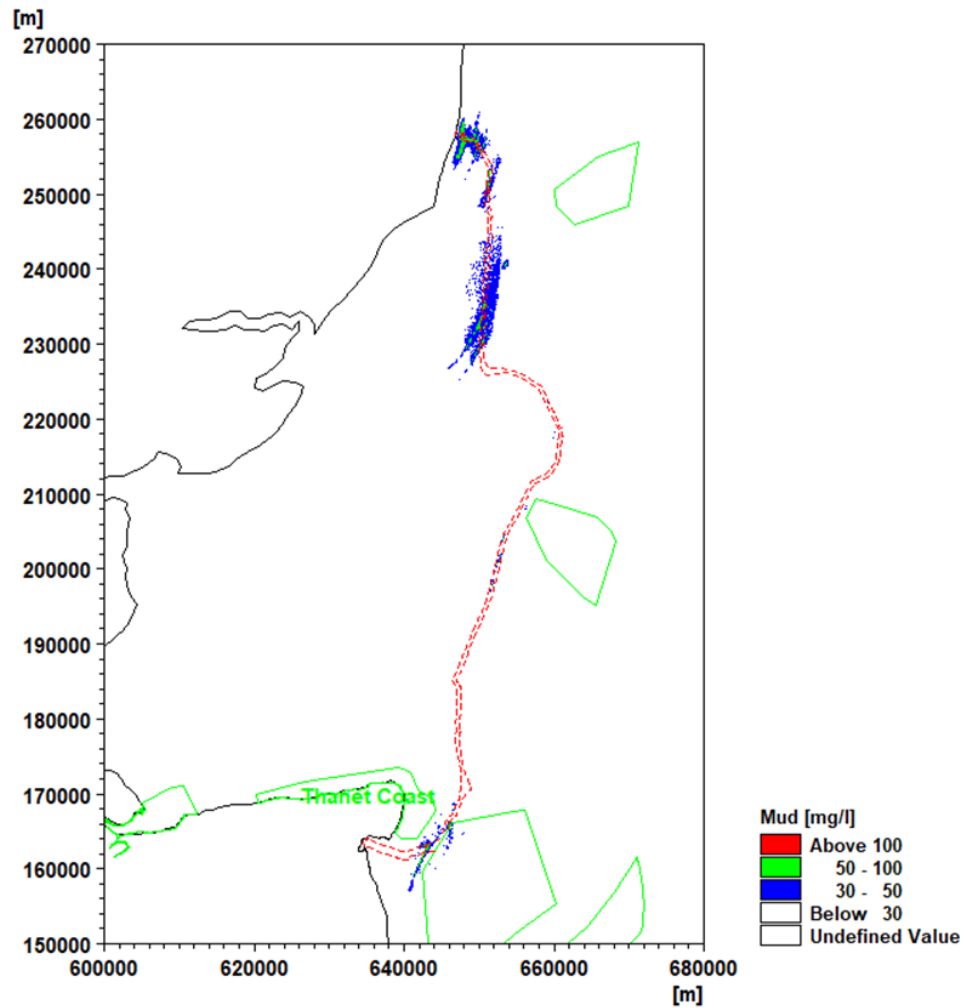
Plate 1.43. Maximum SSC levels over 14-day period for mud (left) and fine sand (right) for installation by ploughjetting
