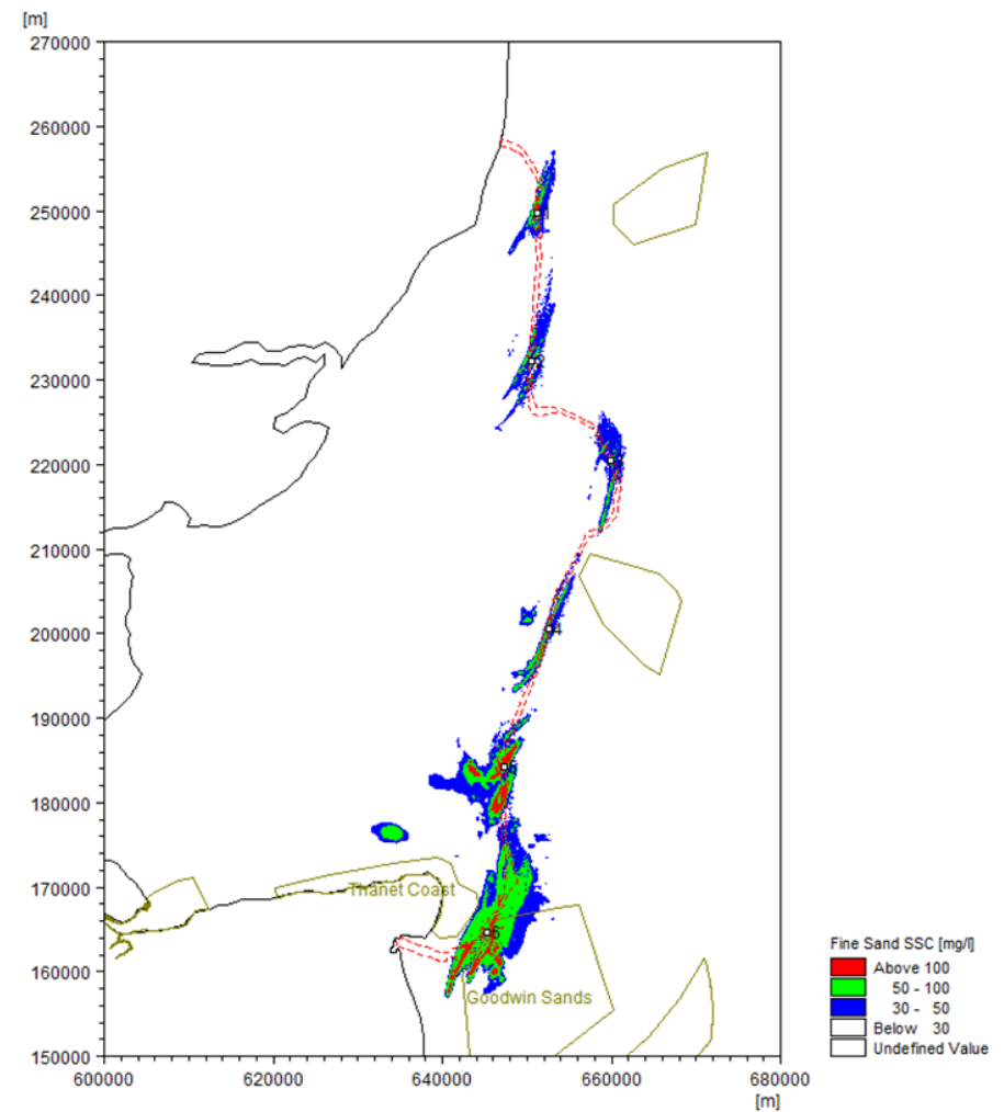
Plate 1.43. Maximum SSC levels over 14-day period for mud (left) and fine sand (right) for installation by ploughjetting
