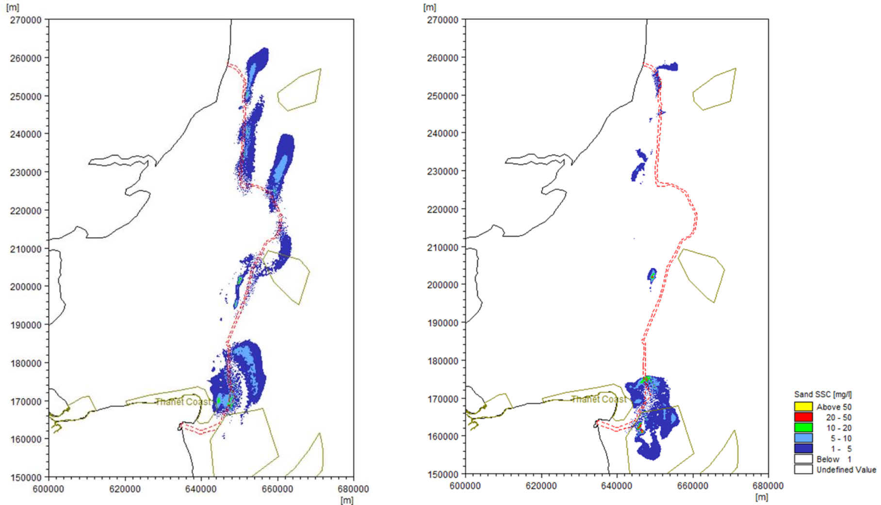
..... jetting installation commencing on spring tides with output at +7 days (left) and +14 days (right) after start of activity
