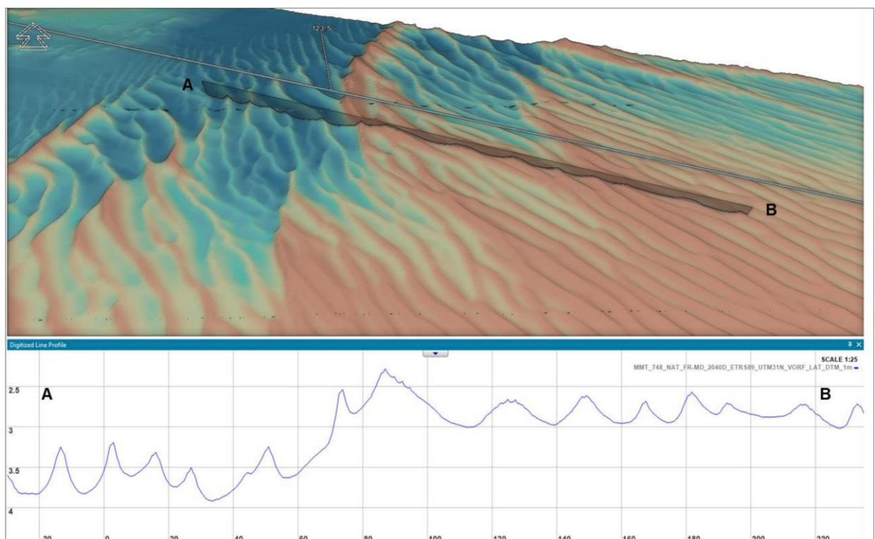
Plate 1.34 Mega ripples Bedforms up to 3.53 m high located near KP 108 (MMT, 2022)
