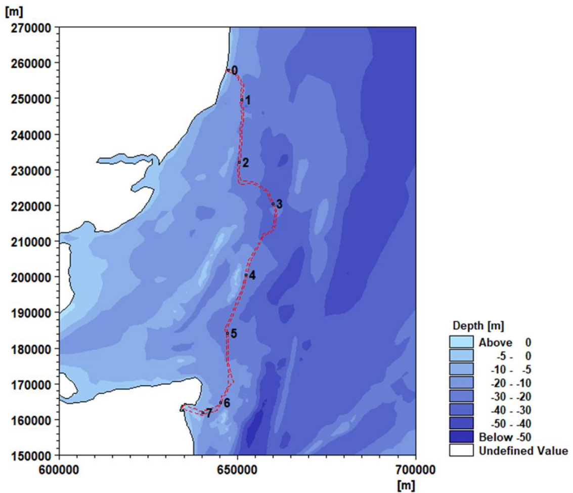
Plate 1.38 Hydrodynamic model bathymetry showing the Offshore Scheme Boundary (red line) and 68 sediment release locations
